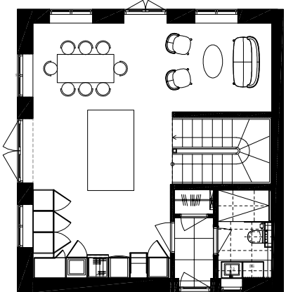
Plan stueetage
