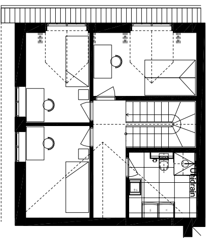
Plan 1. sal
