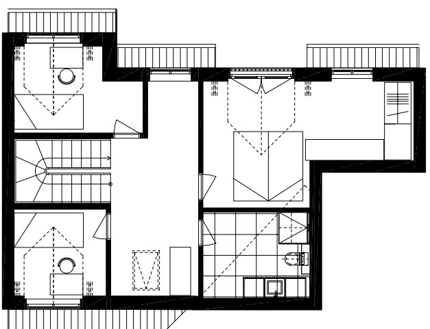
Plan 1. sal
