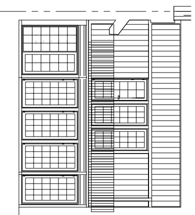
Facade vest
