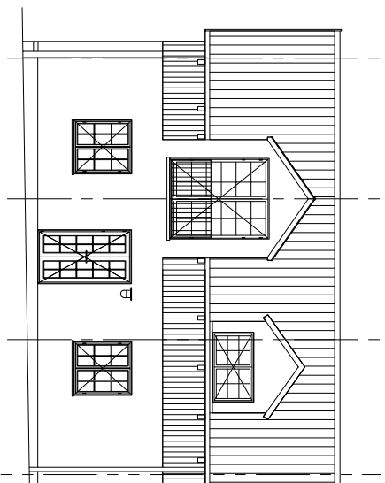
Facade vest
