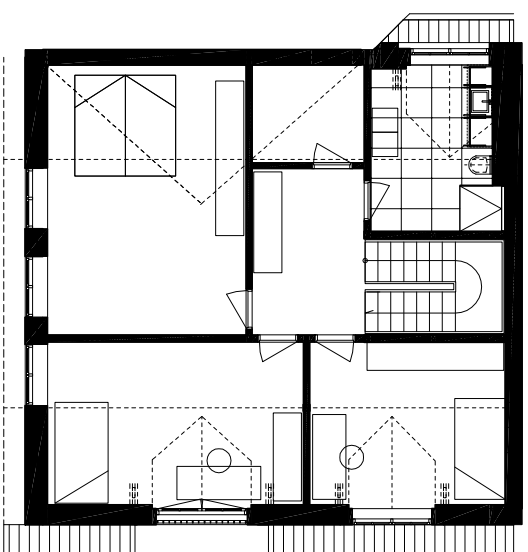
Plan 1. sal
